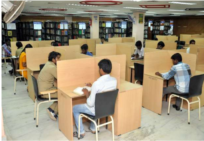
FEAT Library
